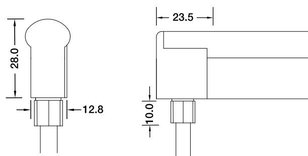
Bottom Entry Connector MJ-SF21-D4-B02SM MJ-SF21-D4-B03SFM
