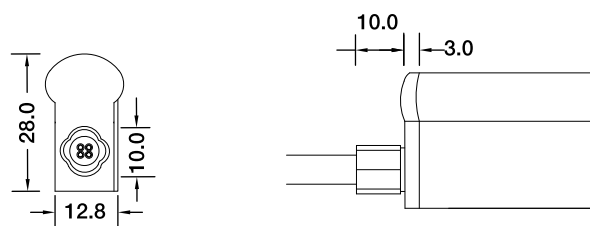
Direct Entry Connector MJ-SF21-D4-D02SM MJ-SF21-D4-D03SFM
