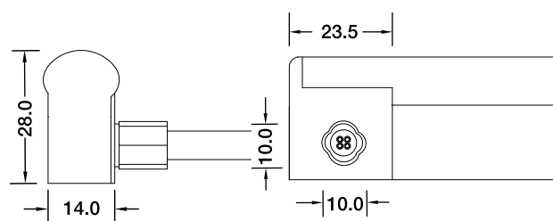
Side Entry Connector MJ-SF21-D4-S02SM MJ-SF21-D4-S03SFM
