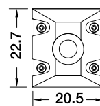
DIY Screw Connector DIY-SC-FR-15-D-01SF/02SM-D4
