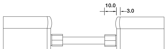
Jumper MJ-SF21-D3-D-JC
