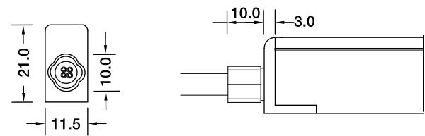
Direct Entry Connector MJ-SF15-RGB-D01/02/03 MJ-SF15-RGB-D01SM MJ-SF15-RGB-D02SF MJ-SF15-RGB-D03SFM
