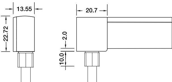
Bottom Entry Connector MJ-SF15-RGB-B01/02/03 MJ-SF15-RGB-B01SM MJ-SF15-RGB-B02SF MJ-SF15-RGB-B03SFM
