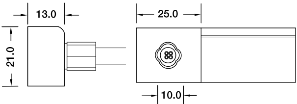
Side Entry Connector MJ-SF15-RGB-S01/02/03 MJ-SF15-RGB-S01SM MJ-SF15-RGB-S02SF MJ-SF15-RGB-S03SFM
