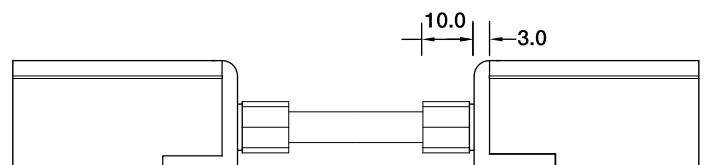
Jumper MJ-SF15-D5-D-JC
