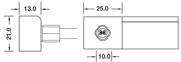
Side Entry Connector MJ-SF15-D5-S02SM MJ-SF15-D5-S03SFM
