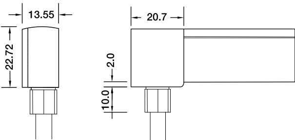
Bottom Entry Connector MJ-SF15-D3-B02SM MJ-SF15-D3-B03SFM
