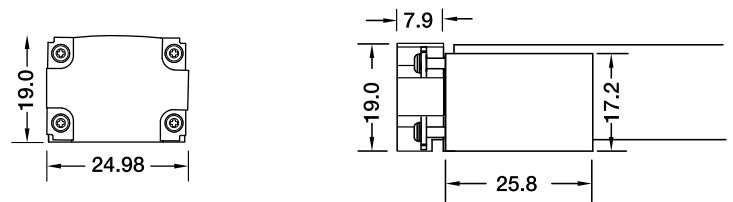
DIY Screw Extension Connector DIY-SC-EXT-16-D3
