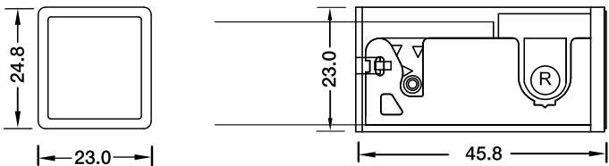
DIY Snap Connector Jumper DIY-SN-FR-16-D3-D-JC
