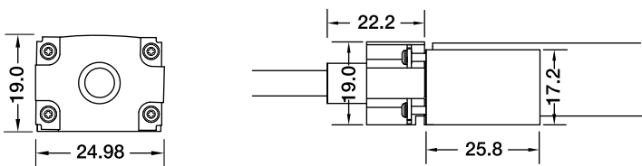
DIY Screw Connector DIY-SC-FR-16-D-01/02-D3
