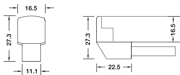
L Shape Entry Connector MJ-SF16-D5-L02SM MJ-SF16-D5-L03SFM
