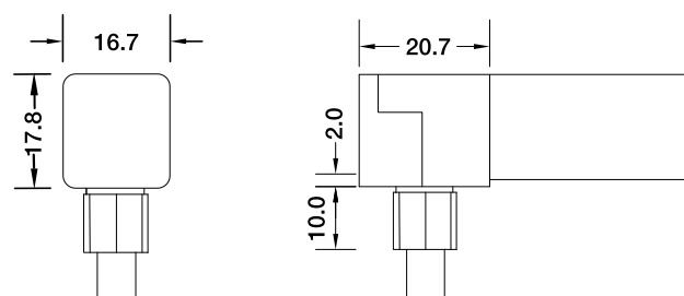
Bottom Entry Connector MJ-SF16-D5-B02SM MJ-SF16-D5-B03SFM
