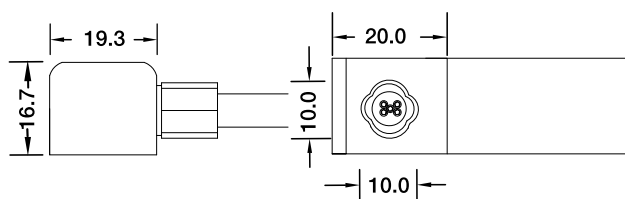
Side Entry Connector MJ-SF16-D5-S02SM MJ-SF16-D5-S03SFM
