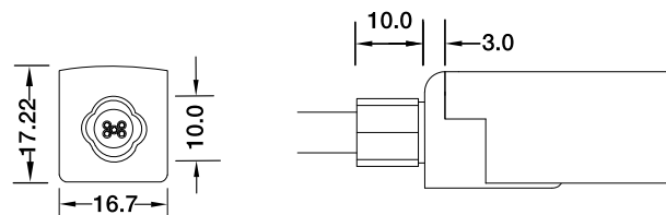
Direct Entry Connector MJ-SF16-D5-D02SM MJ-SF16-D5-D03SFM
