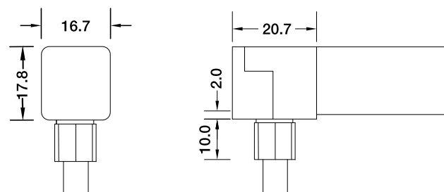
Bottom Entry Connector MJ-SF16-D3-B02SM MJ-SF16-D3-B03SFM
