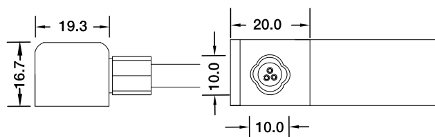
Side Entry Connector MJ-SF16-D3-S02SM MJ-SF16-D3-S03SFM
