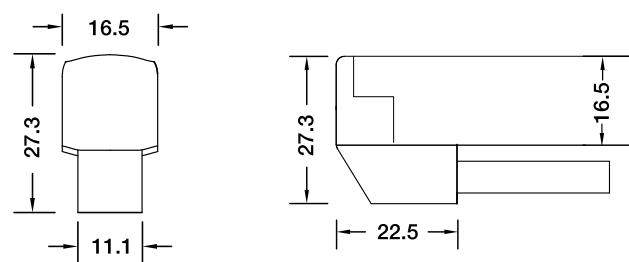
L Shape Entry Connector MJ-SF16-D3-L02SM MJ-SF16-D3-L03SFM
