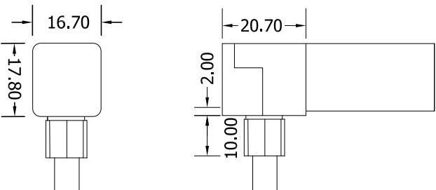
Bottom Entry Connector MJ-SF17-A-B01/02/03 MJ-SF17-A-B01SM MJ-SF17-A-B02SF MJ-SF17-A-B03SFM
