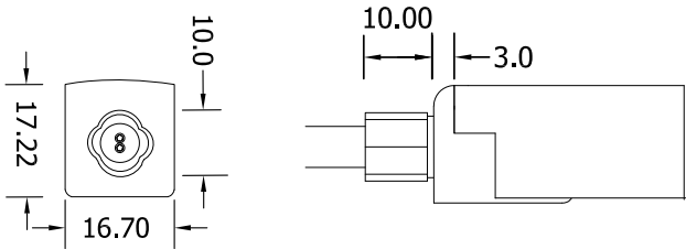
Direct Entry Connector MJ-SF17-A-D01/02/03 MJ-SF17-A-D01SM MJ-SF17-A-D02SF MJ-SF17-A-D03SFM
