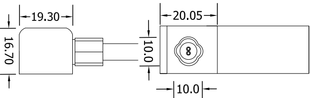
Side Entry Connector MJ-SF17-A-S01/02/03 MJ-SF17-A-S01SM MJ-SF17-A-S02SF MJ-SF17-A-S03SFM
