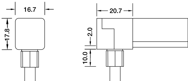
Bottom Entry Connector MJ-SF18-A-S01/02/03 MJ-SF18-A-S01SM MJ-SF18-A-S02SF MJ-SF18-A-S03SFM
