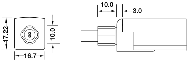
Direct Entry Connector MJ-SF18-A-D01/02/03 MJ-SF18-A-D01SM MJ-SF18-A-D02SF MJ-SF18-A-D03SFM
