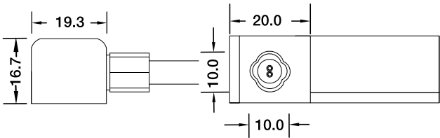
Side Entry Connector MJ-SF18-A-S01/02/03 MJ-SF18-A-S01SM MJ-SF18-A-S02SF MJ-SF18-A-S03SFM
