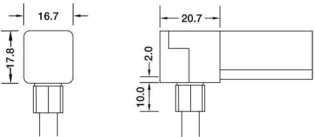
Bottom Entry Connector MJ-SF18-DW-S01/02/03 MJ-SF18-DW-S01SM MJ-SF18-DW-S02SF MJ-SF18-DW-S03SFM
