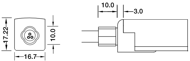
Direct Entry Connector MJ-SF18-DW-D01/02/03 MJ-SF18-DW-D01SM MJ-SF18-DW-D02SF MJ-SF18-DW-D03SFM
