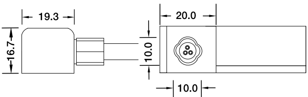
Side Entry Connector MJ-SF18-DW-S01/02/03 MJ-SF18-DW-S01SM MJ-SF18-DW-S02SF MJ-SF18-DW-S03SFM
