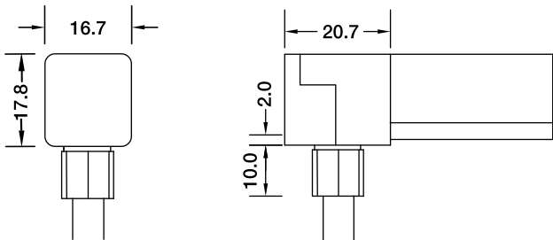
Bottom Entry Connector MJ-SF18-D3-S02SM MJ-SF18-D3-S03SFM
