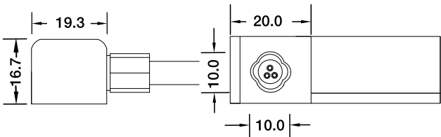
Side Entry Connector MJ-SF18-D3-S02SM MJ-SF18-D3-S03SFM
