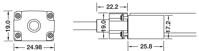
DIY Screw Connector DIY-SC-FR-16-D-01SF/02SM-D3
