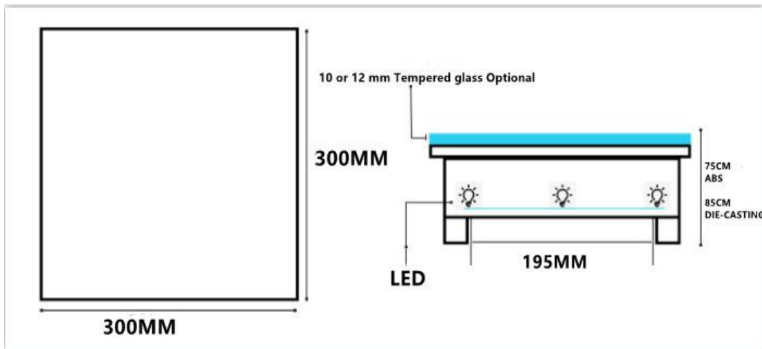
DIE-CASTING HOUSING
