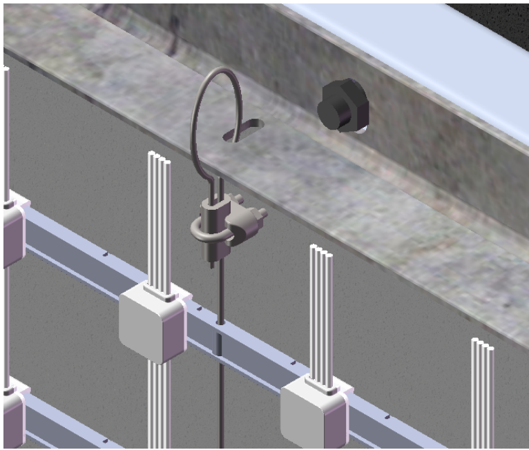
Detail view 1
