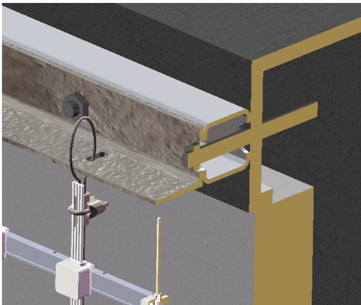
Detail view 5
