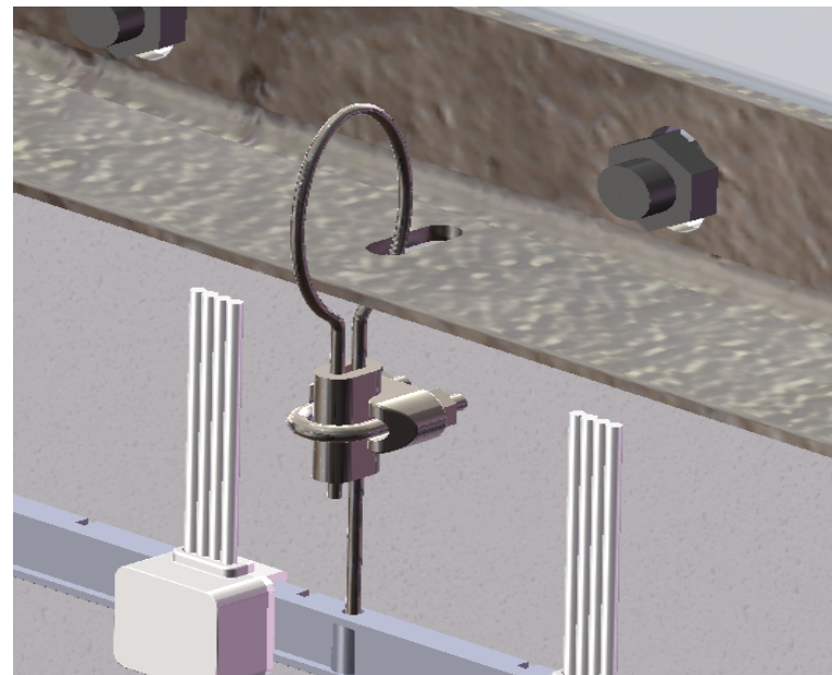
Detail view 4
