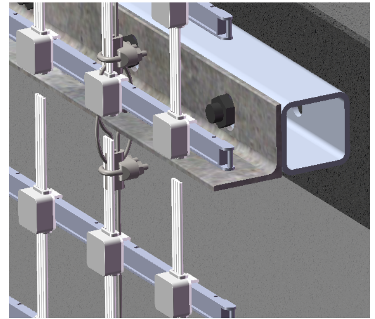
Detail view 3
