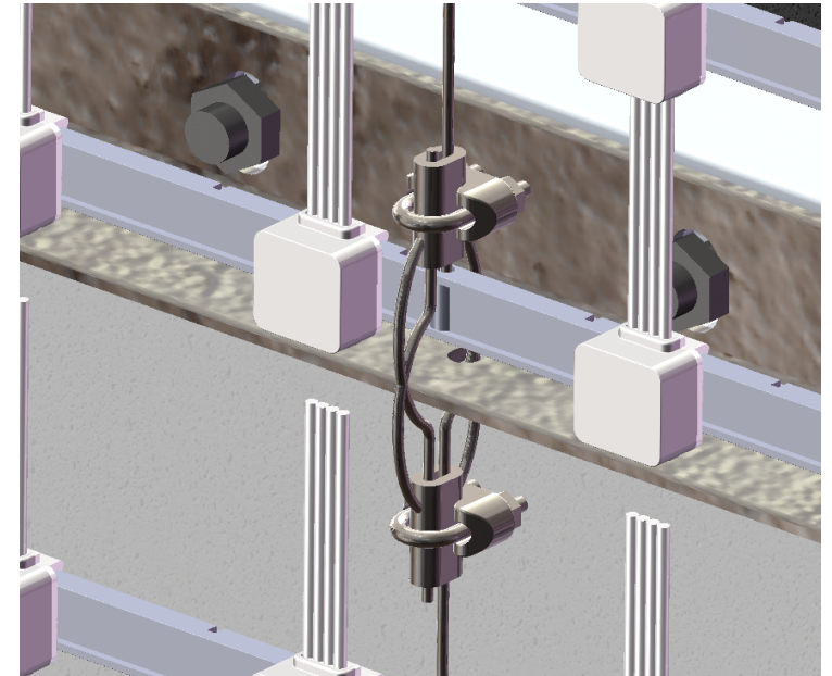
Detail view 6
