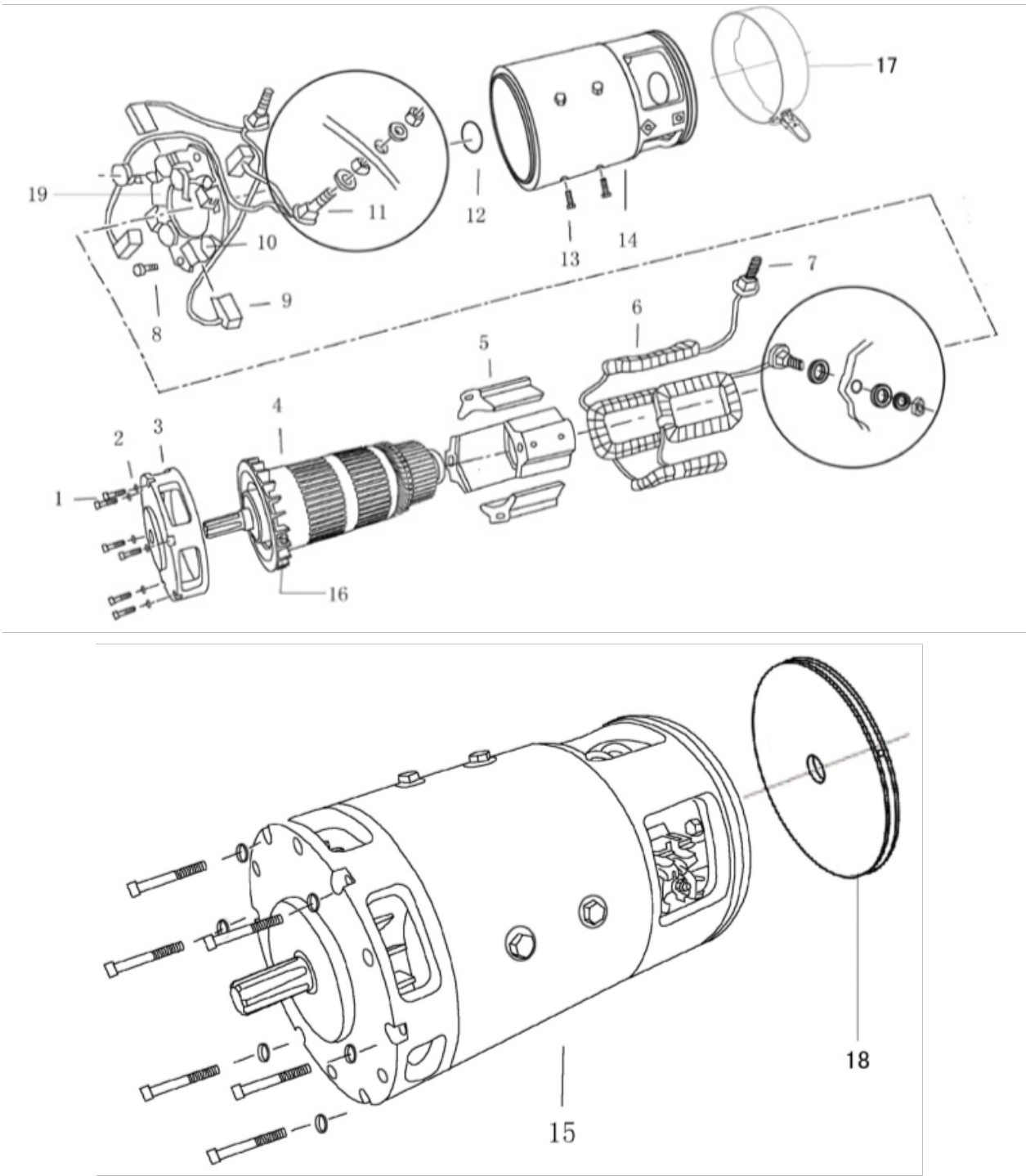
48 V, 3 KW Series Motor
