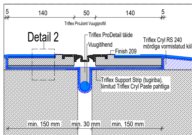
Detail 1, Triflex ProJoint
