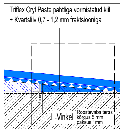
Detail 3, Triflex ProJoint (Triflex Cryl Paste Kiil)
