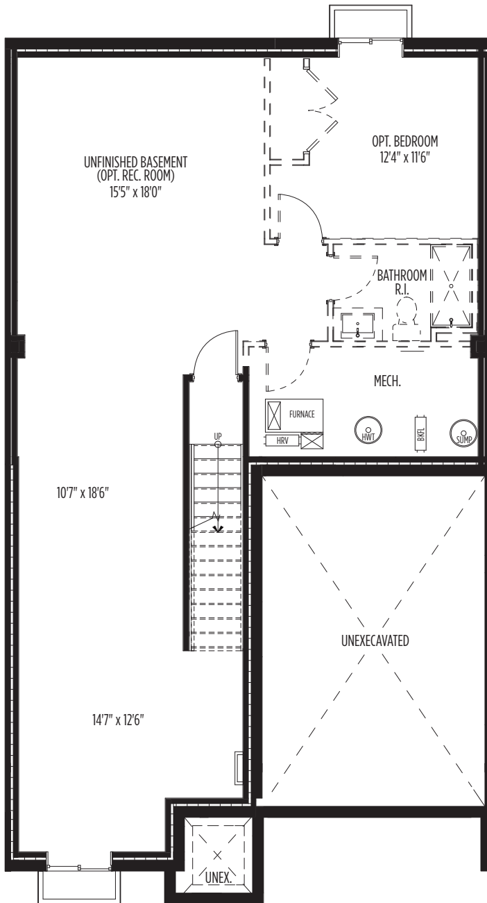
Basement Plan
