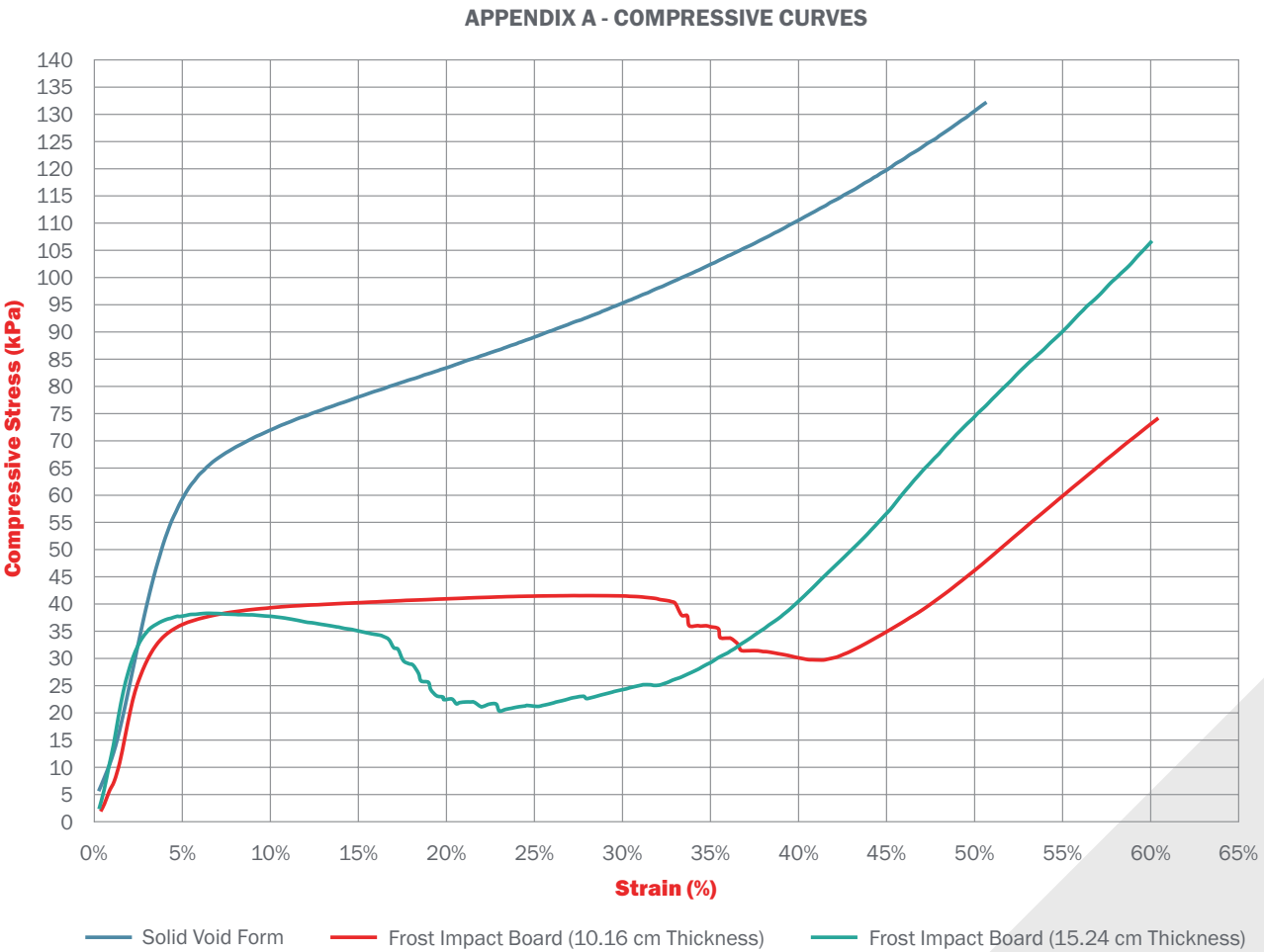
Figure 1 - Compressive Stress vs Strain Curves
