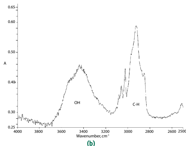
Fig. 6: FTIR spectra for GFRP in the Joffe Bridge: (a) in-service GFRP; and (b) control GFRP
