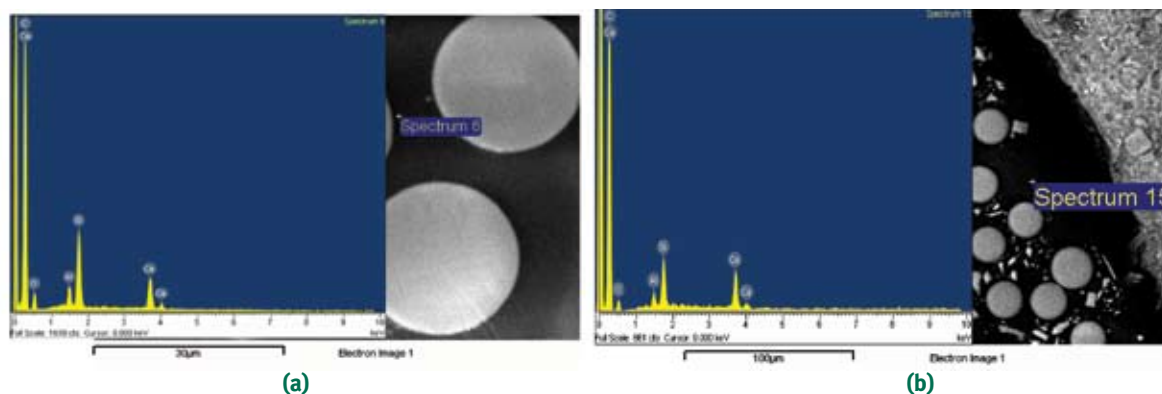
Fig. 5: EDX scans for the polymer matrix from the Joffe Bridge: (a) in-service matrix; and (b) control matrix
