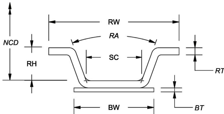
V-RETAINER PROFILE
