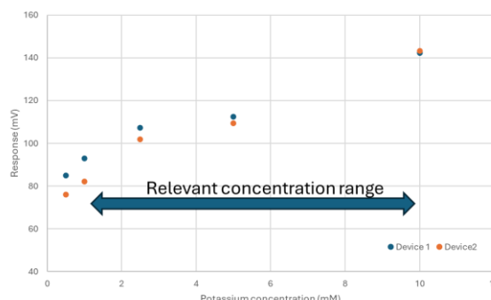
Example data of sensor response to potassium levels
