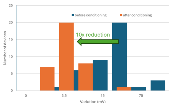
Voltage sweep repeatability – effect of conditioning
