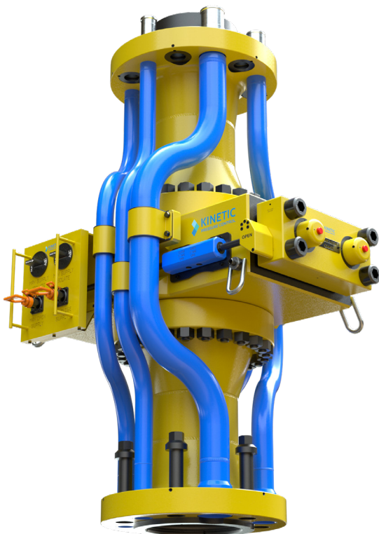
19.25" Bore MRV c/w Cameron SLB LK 3.5 Riser Connection
