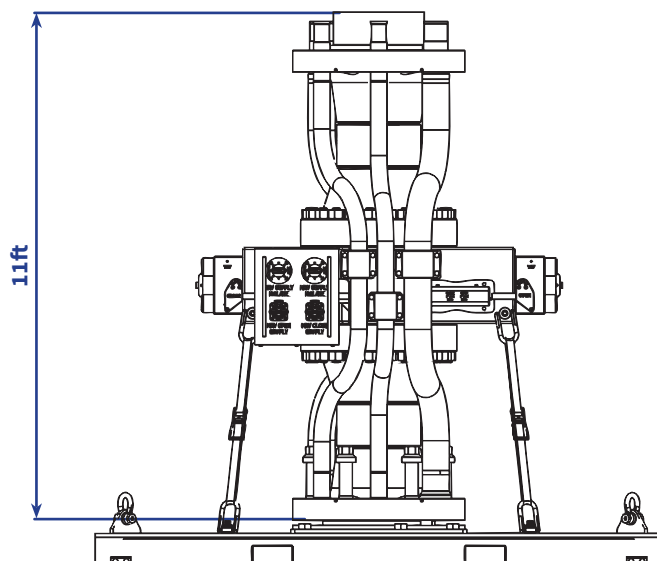
GV19A301 (MRV with LK3.5 Crossovers shown)
