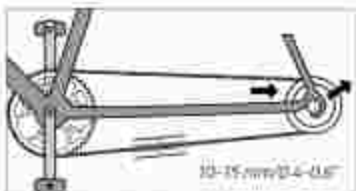
Illustr: Chain tension (mm/0.4")
