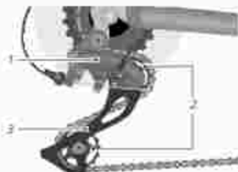
Illustr: Moving components of a derailleur shifting system (rearview)
