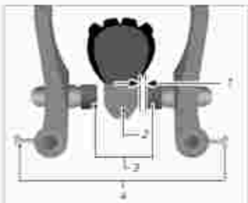
Illustration: Brake block holder distance (spring)
