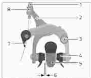
Illustr. Racejg bike rim brake assembly
