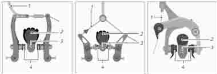
Illustr.: Mechanical rim brakes (source:W)
