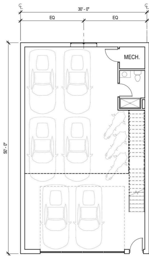
UNIT 1ST FLOOR 1,500 SF SCALE: 1/8" = 1' - 0"
