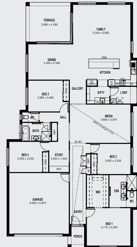
DESIGNER PLUS - 273.60m 2 / 29.45sq
