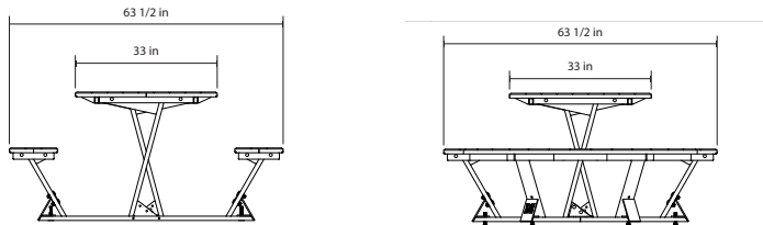
END VIEW
