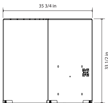
SIDE VIEW - TALL
