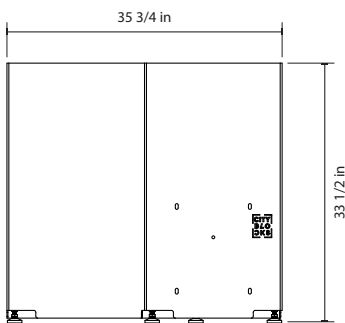
SIDE VIEW - TALL
