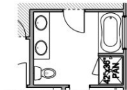
OPT. OWNERS BATH #2
