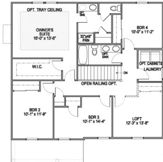
ALTERNATE 2ND FLOOR
