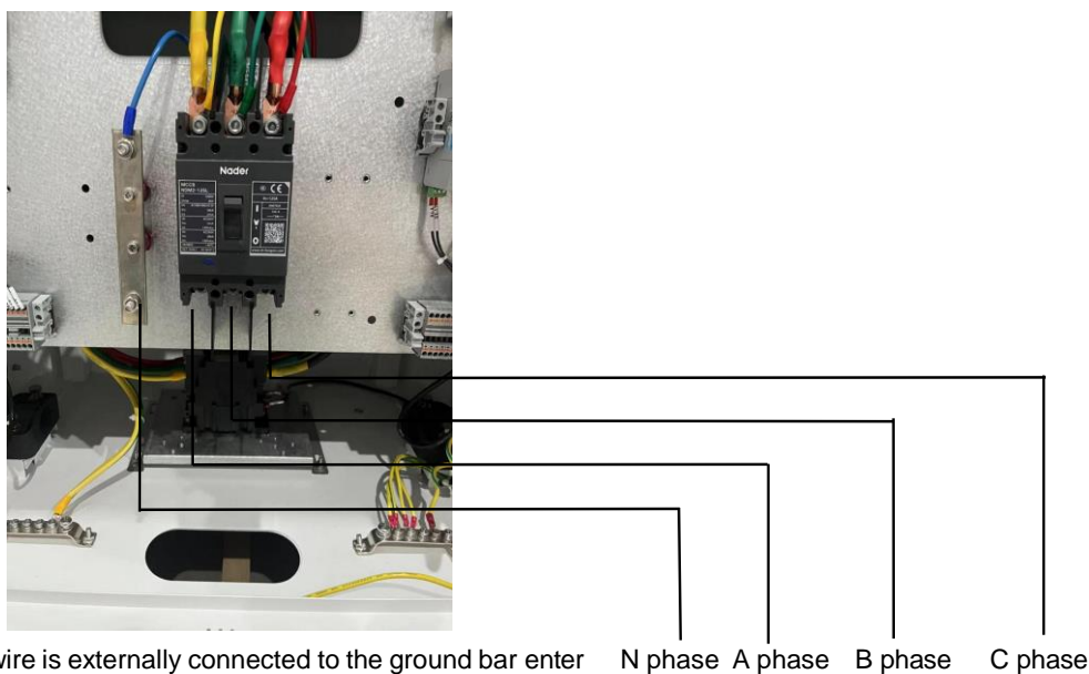
Figure 5-3-1 Cable Access
