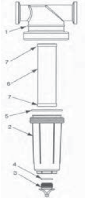
Replacement Parts - MLST100 & MLST150
