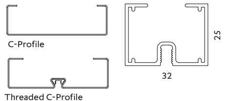
Threaded C-Profile
