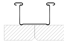
Direct Fix Furring Channels
