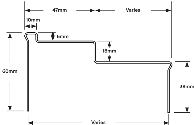
ISD Frame to suit 47mm Door
