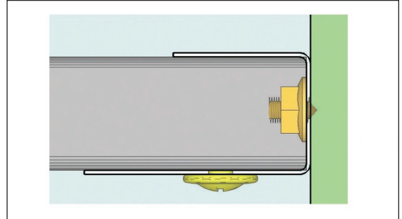
M40/M42 INSTALLATION EXAMPLE
