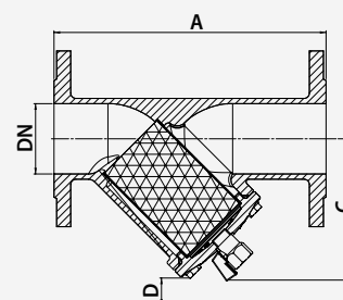
Type Y333P flanged
