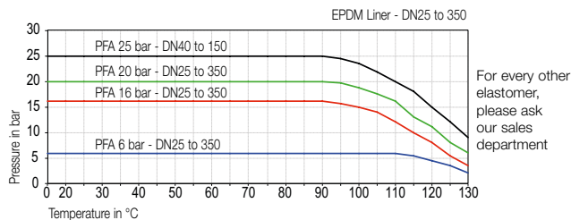
PRESSURE/TEMPERATURE CHART
