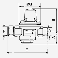
Type 7EP female/male
