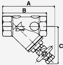
Type Y222P threaded
