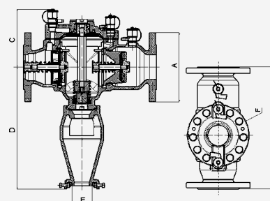
Type BA4760 flanged
