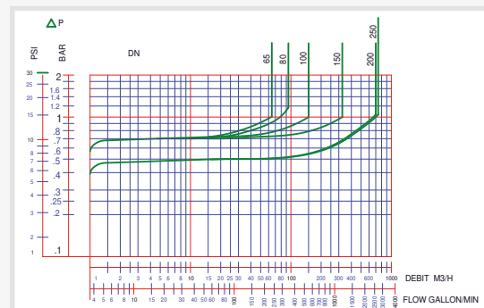
HEADLOSS CHART
