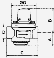
Type 7BIS female/female
