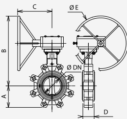
Tilis Lugged Gearbox
