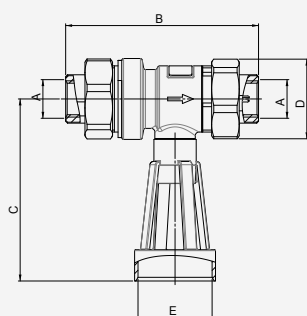
Type CA 2096 female/female
