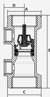
Type EA291NF female/female
