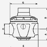
Type 9BIS female/female
