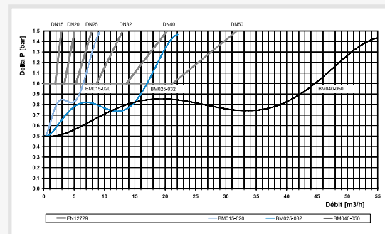
HEADLOSS CHART
