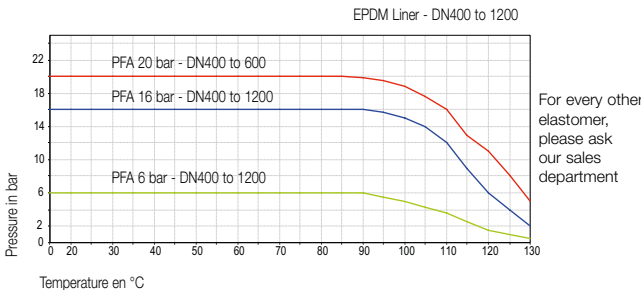
PRESSURE/TEMPERATURE CHART
