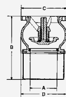
with flange
