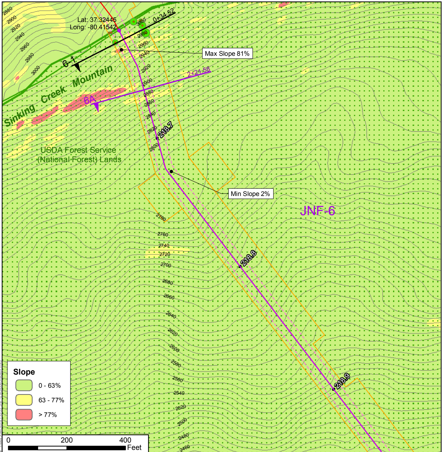
Figure 53, Site 6 Jefferson National Forest Slope Stability Map and Representative Cross Section Locations 03-12-18
