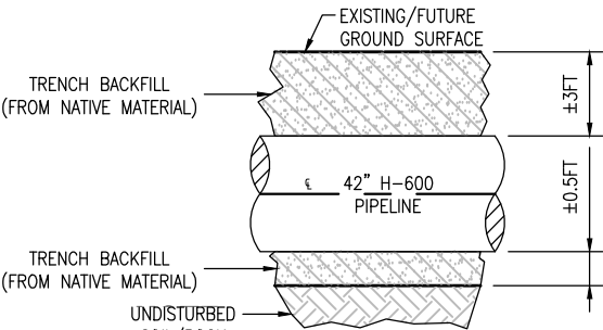
TYPICAL TRENCH BACKFILL (NOT TO SCALE)
