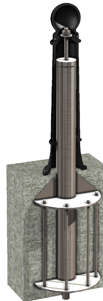
INSTALLED BOLLARD SLEEVE S10/S20 Mounting Shown
