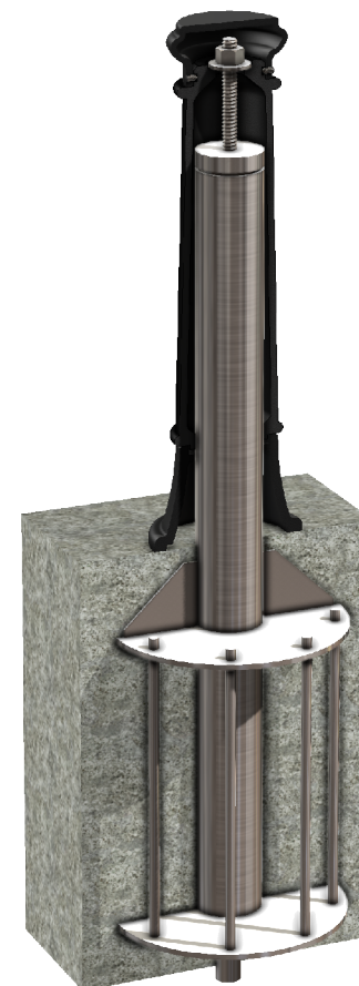
INSTALLED BOLLARD SLEEVE S10/S20 Mounting Shown
