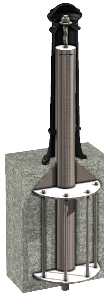
INSTALLED BOLLARD SLEEVE S10/S20 Mounting Shown
