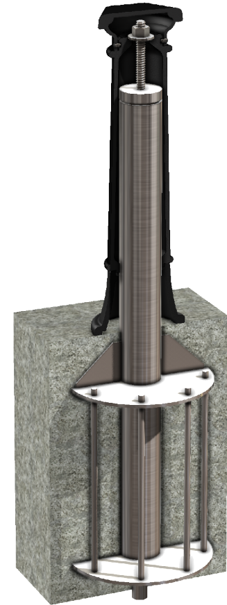
INSTALLED BOLLARD SLEEVE S10/S20 Mounting Shown
