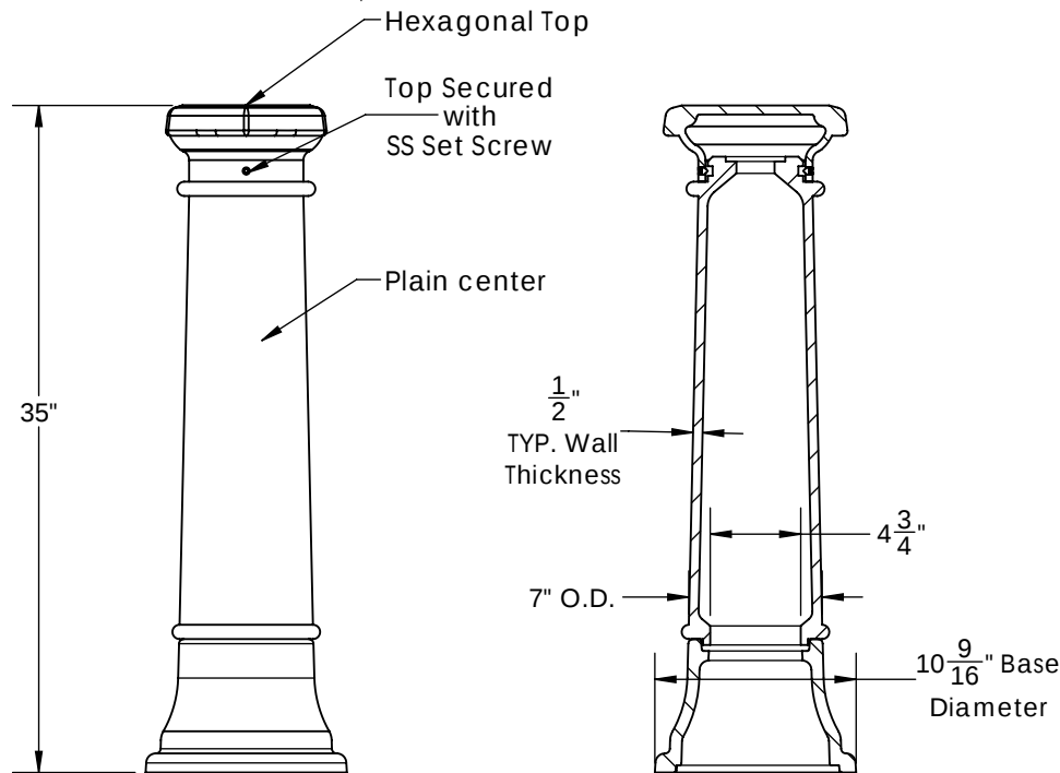
SIDE VIEW
