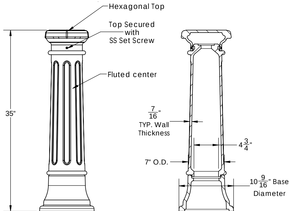
SIDE VIEW
