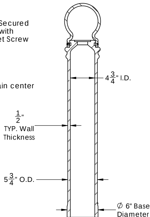
SECTION
