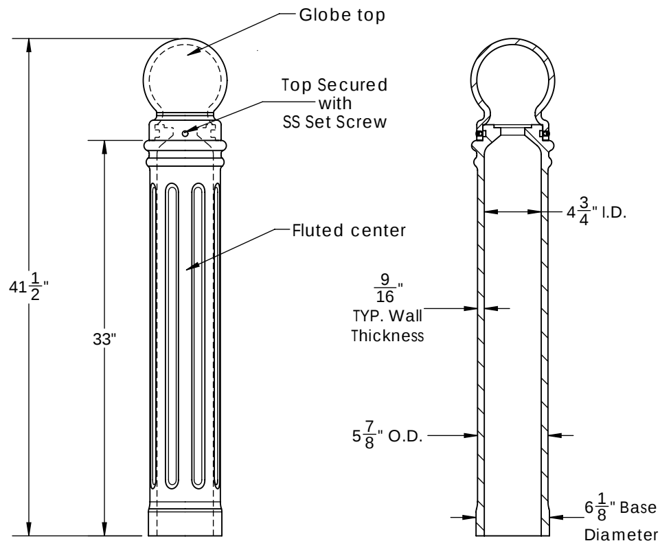
SIDE VIEW
