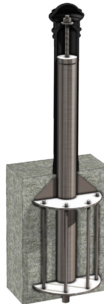
INSTALLED BOLLARD SLEEVE S10/S20 Mounting Shown
