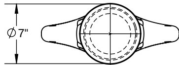
TOP VIEW Cast Iron Sleeve
