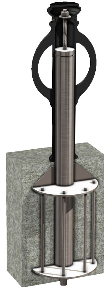
INSTALLED BOLLARD SLEEVE S10/S20 Mounting Shown
