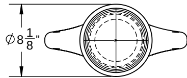
TOP VIEW Cast Iron Sleeve
