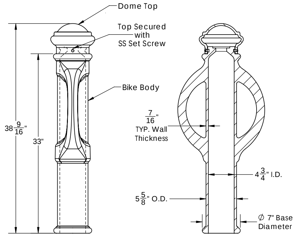
SIDE VIEW
