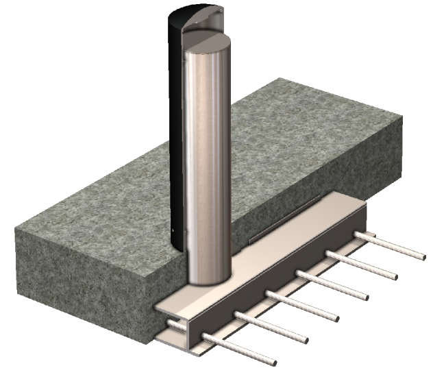
INSTALLED BOLLARD SLEEVE K4M30 Shallow Mounting
