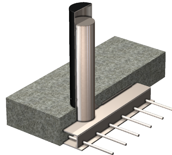
INSTALLED BOLLARD SLEEVE K4M30 Shallow Mounting
