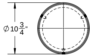
TOP VIEW A-36 Mild Steel Sleeve
